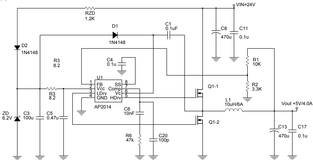
Single Supply 24V Input
